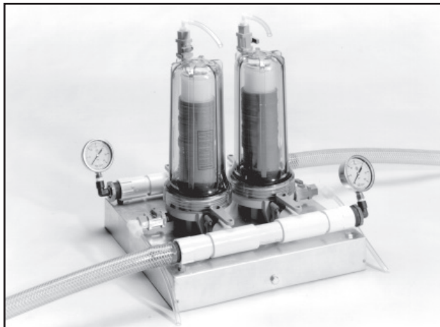
FS6000 Pre-Filter Module – 50 GPM
